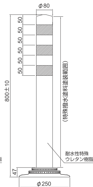
PC-80PFR(G)W-N
