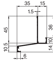
HA-35-L27 (出幅35mm)
