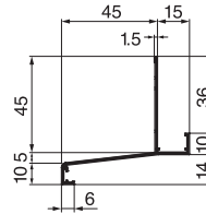
HA-45-L27 (出幅45mm)
