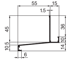
HA-55-L27 (出幅55mm)
