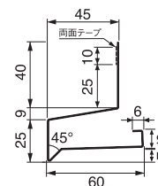
HF-A4560 (出幅45mm)
