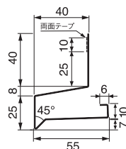
HF-A4055 (出幅40mm)
