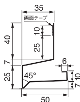
HF-A3550 (出幅35mm)
