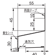
WMF-N55(出幅55mm)
