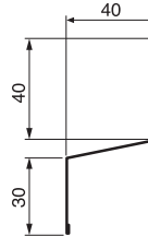
WSF-40 (出幅40mm)
