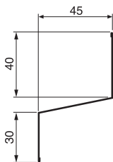
WSF-45 (出幅45mm)
