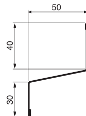
WSF-50 (出幅50mm)
