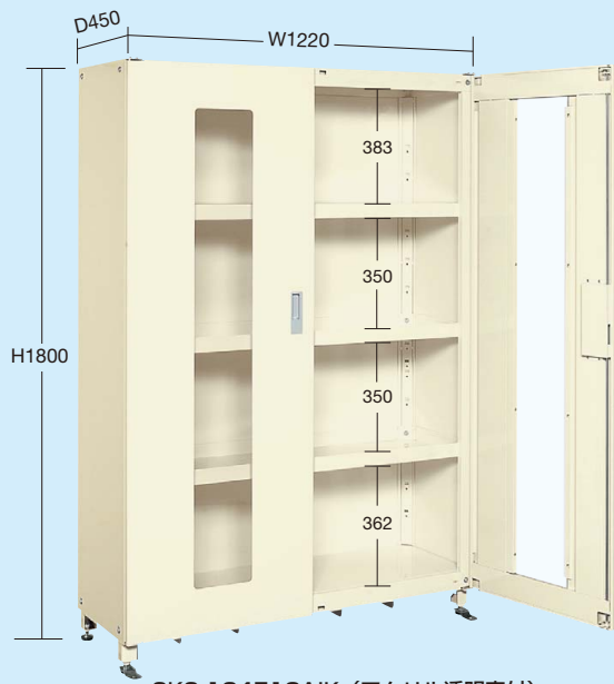
SKS-124518AIK (アクリル透明窓付)
